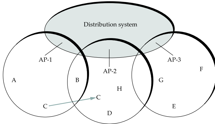
Figure 2.44 Node mobility.
