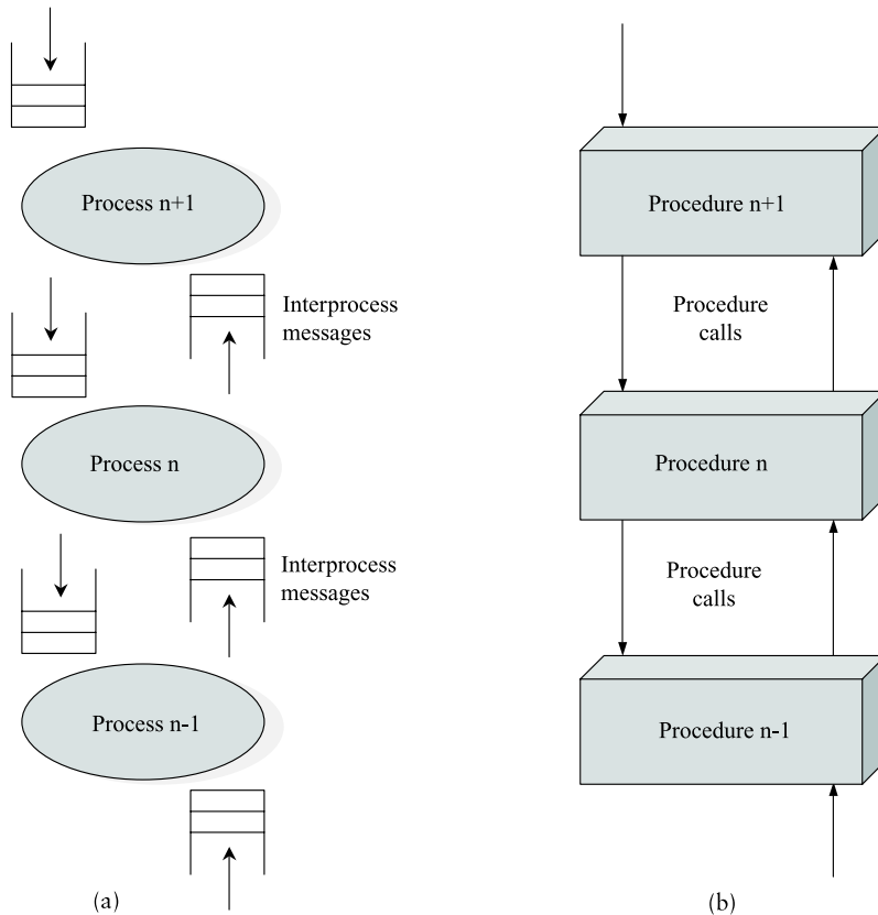
Figure 1.16 Alternative process models: (a) process-per-protocol; (b) process-per-message.
