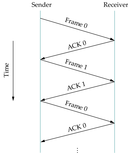
Figure 2.23 Timeline for stop-and-wait with 1-bit sequence number.
