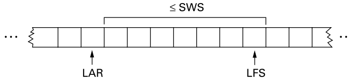
Figure 2.25 Sliding window on sender.
