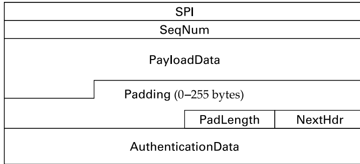
Figure 8.17 IPsec’s ESP format.
