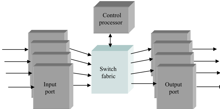
Figure 3.25 A 4 \times 4 switch.
