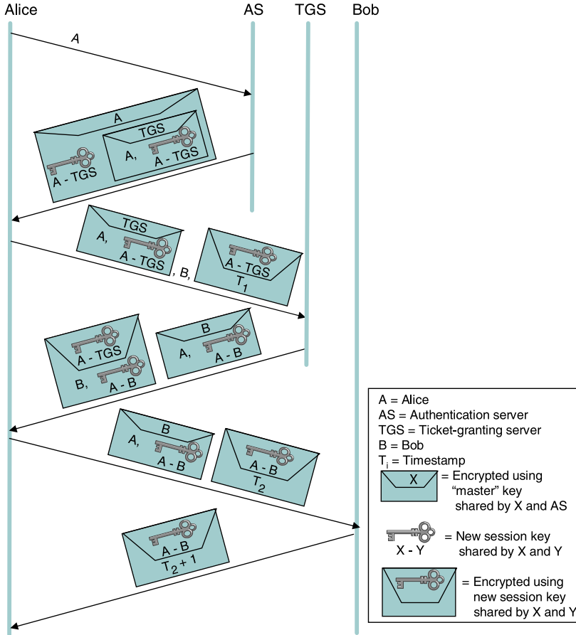
Figure 8.11 Kerberos authentication.
