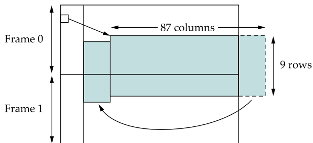
Figure 2.18 SONET frames out of phase.
