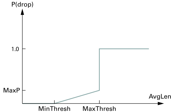
Figure 6.17 Drop probability function for RED.
