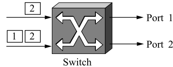
Figure 3.26 Simple illustration of head-of-line blocking.
