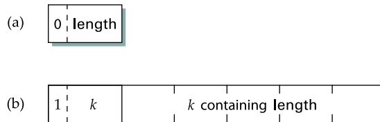
Figure 7.9 ASN.1/BER representation for length: (a) 1 byte; (b) multibyte.
