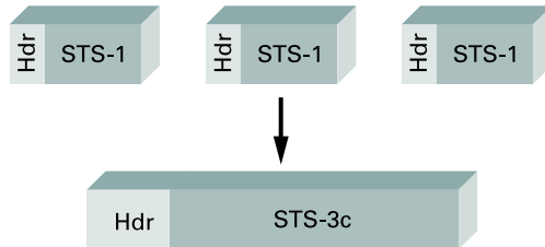
Figure 2.17 Three STS-1 frames multiplexed onto one STS-3c frame.
