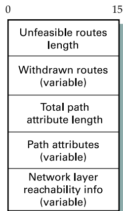
Figure 4.31 BGP-4 update packet format.
